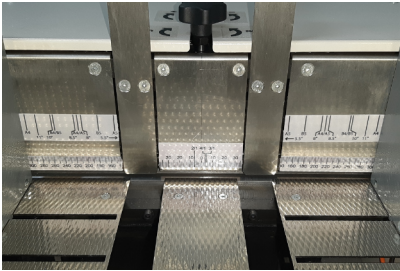
Easy setting of the feeder with capacity up to 150 mm
